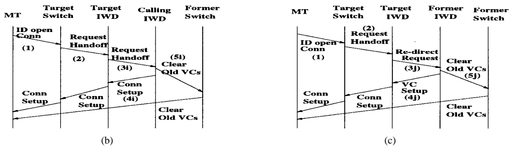
Fig. 31. IWD's handoff scheme: (a) architecture; (b) connection reroute signal flow; and (c) connection extension signal flow.
