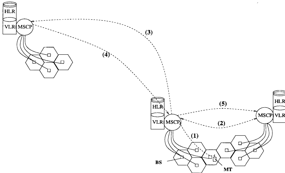
Fig. 25. Two-tier database scheme.
