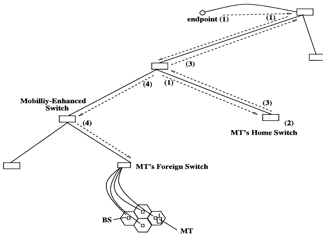
Fig. 29. Integrated location resolution.
