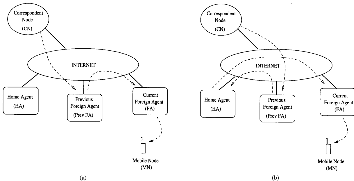
Fig. 23. Mobile IP smooth handoff: (a) fresh binding at previous FA and (b) no fresh binding at previous FA.
