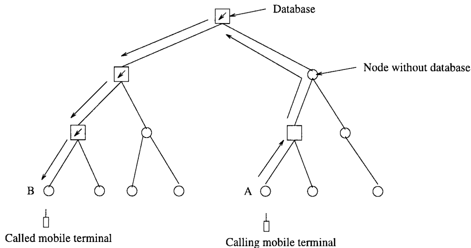
Fig. 14. Distributed database architecture.
