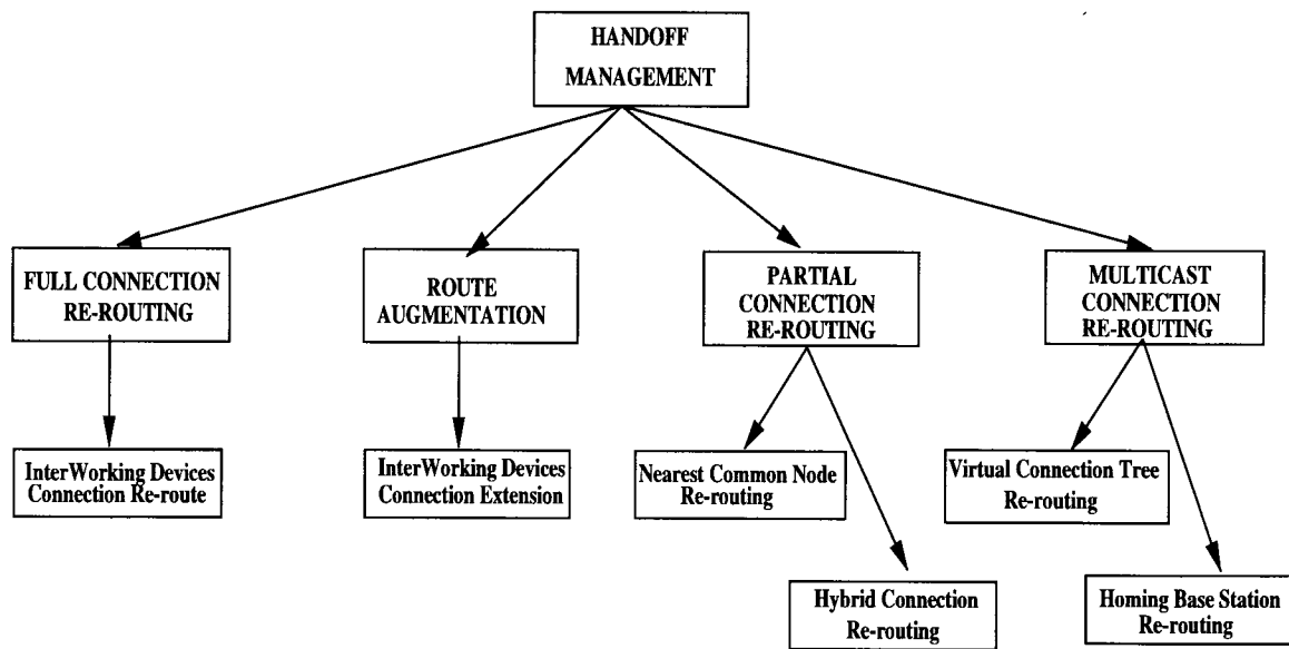
Fig. 30. WATM handoff management techniques.
