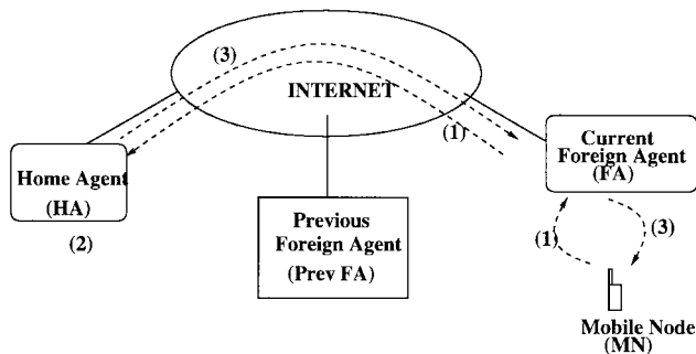
Fig. 21. Mobile IP location registration.
