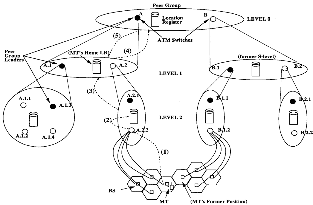
Fig. 26. WATM location registers scheme.
