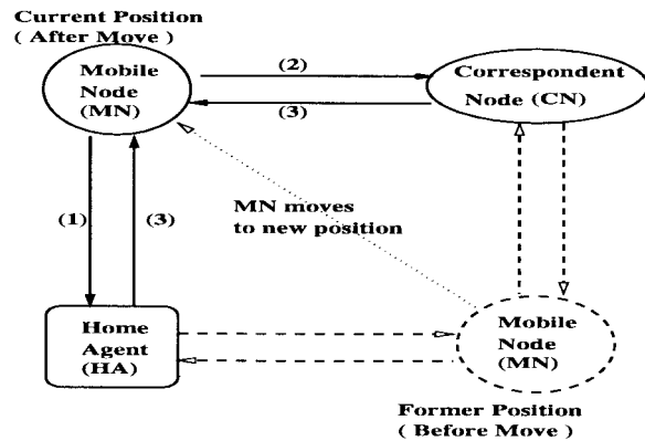
Fig. 22. Mobile IP location management operations.
