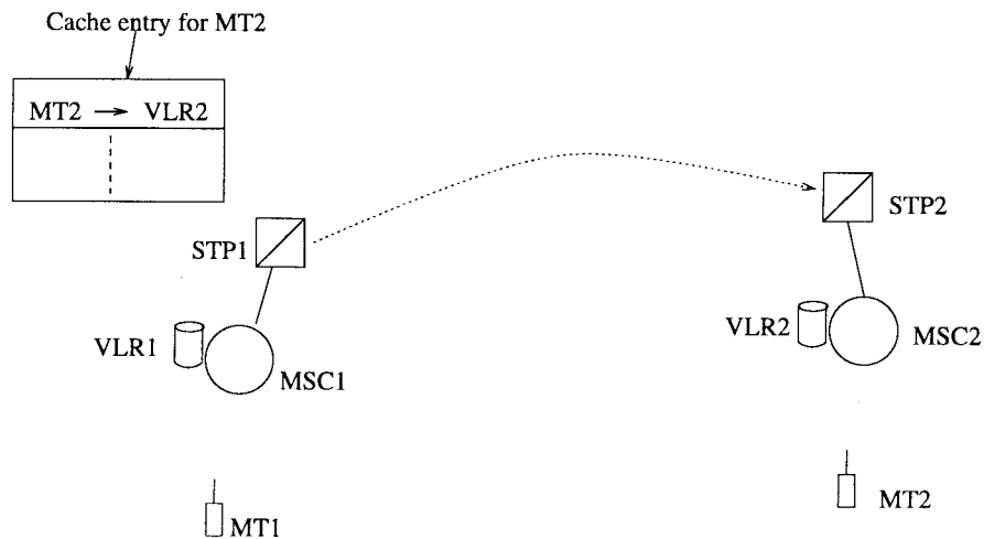
Fig. 9. Per-user location caching scheme.
