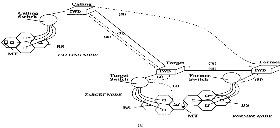
Fig. 30. WATM handoff management techniques.
