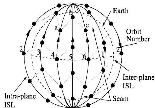
Fig. 36. LEO satellite network with seam.
