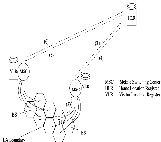
Fig. 7. Location registration procedures.
