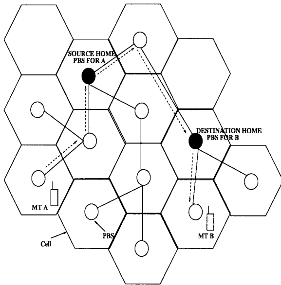
Fig. 35. Homing algorithm handoff routing procedure.
