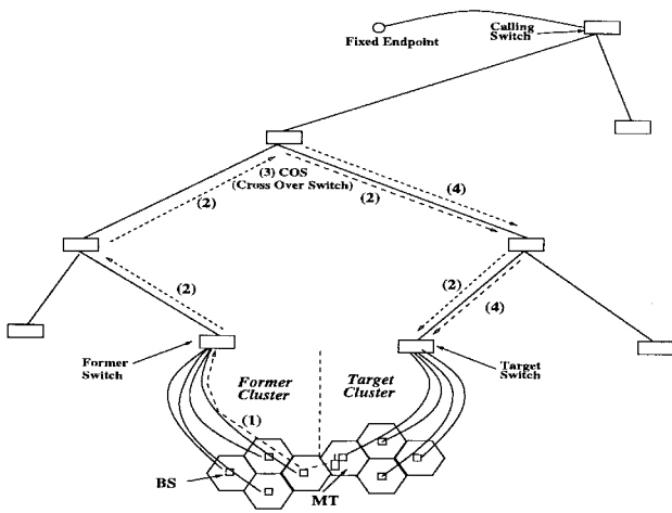
Fig. 33. Hybrid connection rerouting procedure.
