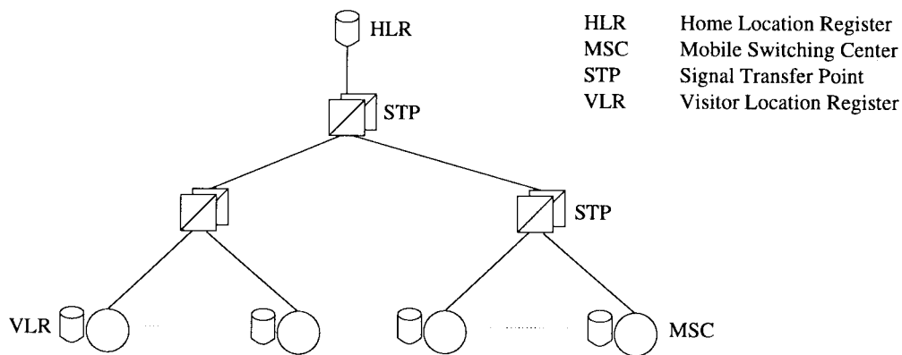
Fig. 6. SS7 signaling network.
