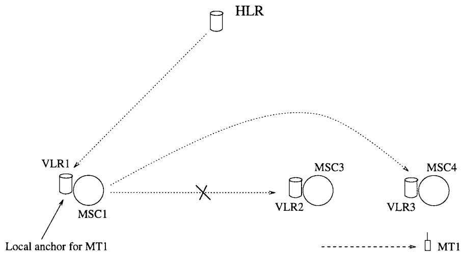
Fig. 11. Local anchoring scheme.
